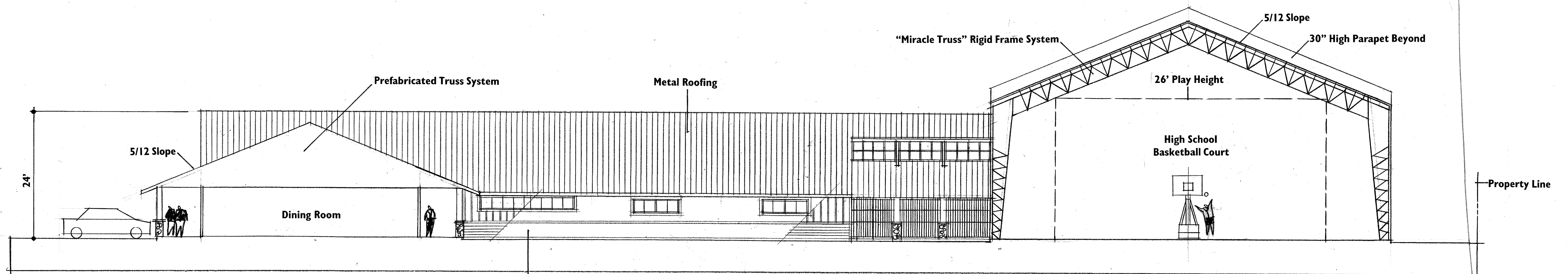
Cross Section B-B
